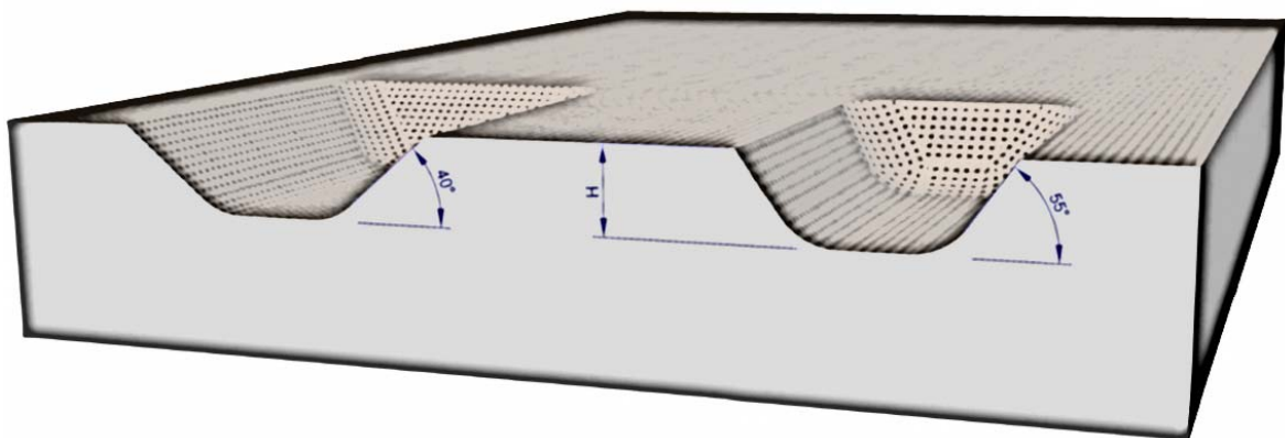
Figure 2 - Examples of acceptable and unacceptable sloped excavations in good ground conditions with no water
